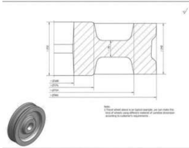
Drawing of rail wheel
